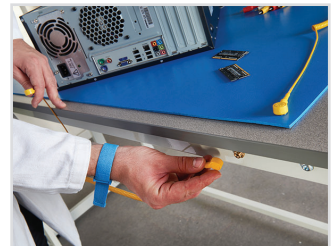
Each workbench is fitted with 4mm Socket
